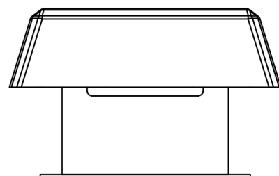
SPEECH GUARD G2 PLENUM RETURN AIR SILENCER
